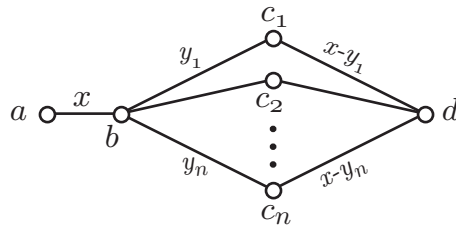
Figure 6: A typical magic labeling of G_f .
