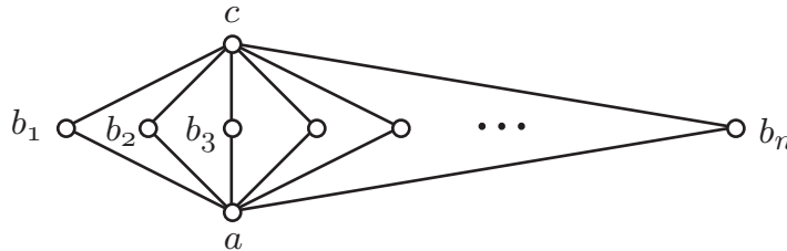
Figure 4: \text{Ext}(P_3, g) = K(2, n)
