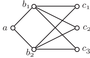
Figure 3: \text{Ext}(P_3, f)
