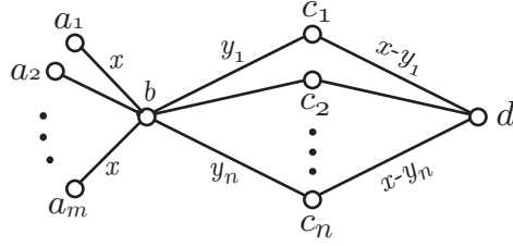
Figure 7: A typical magic labeling of G_f .
