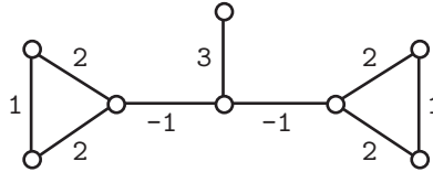
FIGURE 4. IM(G) = \mathbb{N} - \{2, 3\} .
